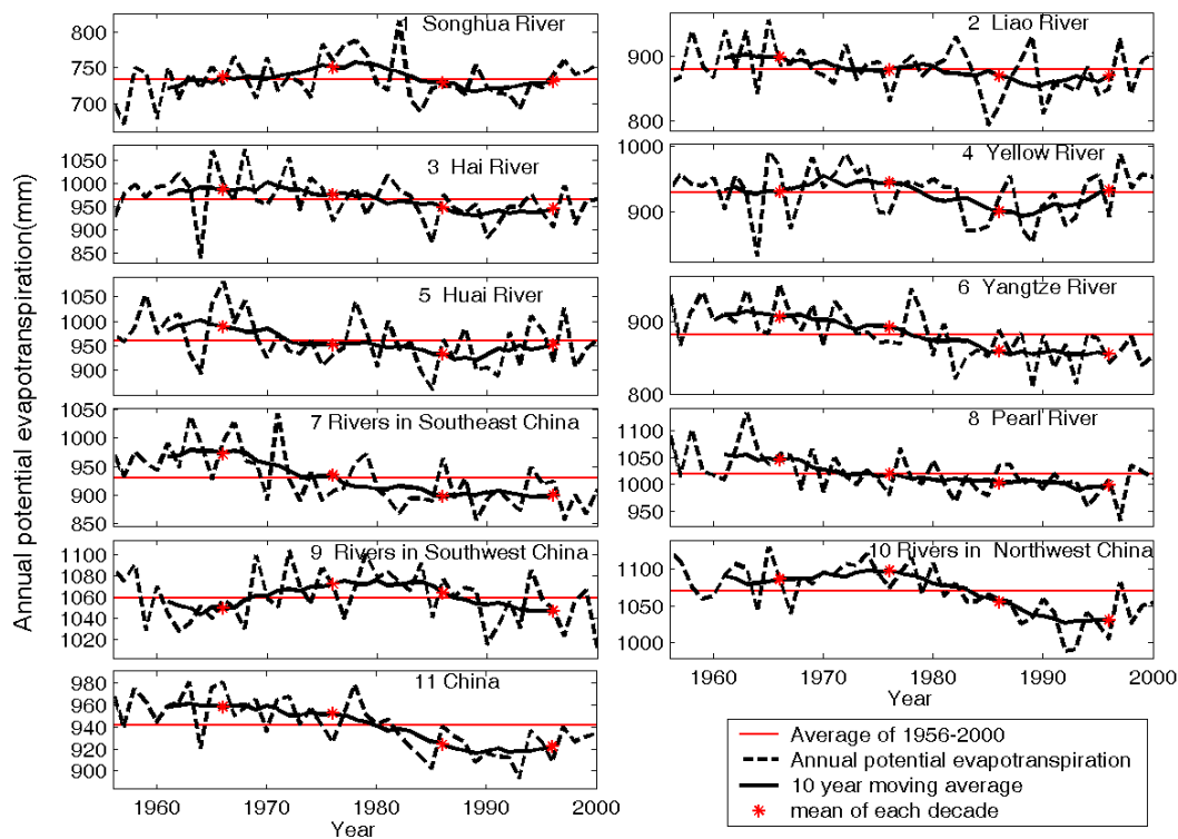
Figure 3 The time series of annual potential evapotranspiration of 10 river basins and China during 1956 to 2000. The thin line represents the normal during this period, the dash line denotes the annual potential evapotranspiration, the thick line is the 10 year moving mean, and star (*) denotes the mean of each decade.
